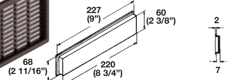
Air Ventilation Grill , with flanged rim • Ventilation area cm 2 : 60 Material: plastic
