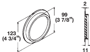
Air Ventilation Cap , recess-mounted, with flanged rim Ventilation area cm 2 : 50.0 Material: plastic
