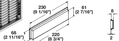
Air Ventilation Grill , with flanged rim • Ventilation area cm 2 : 42.24 Material: plastic
