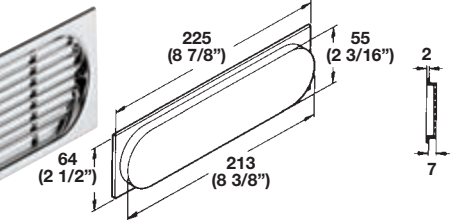
Air Ventilation Grill , with flanged rim and oval recess section, without holes; mounts with adhesive • Ventilation area cm 2 : 45.0 Material: plastic
